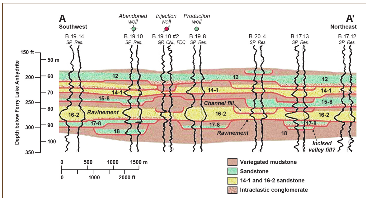
Cross-section through the pilot test area of the Citronelle Field shows the challenge of geologic complexity in fields where CO 2 flooding is being considered. Well B-19-10 #2 is the CO 2 injection well.
