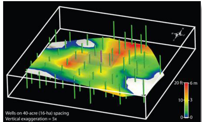
Depiction of reservoir model used for simulation of CO 2 flooding
